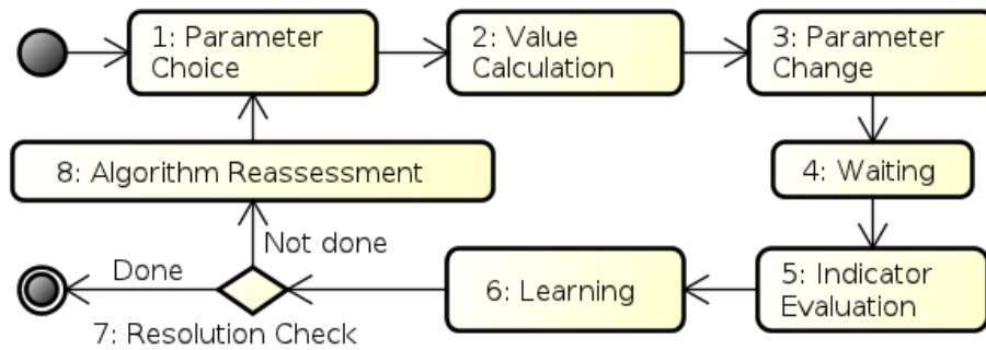
Figure 4.4: The adaptation process followed by the Qualia framework.
