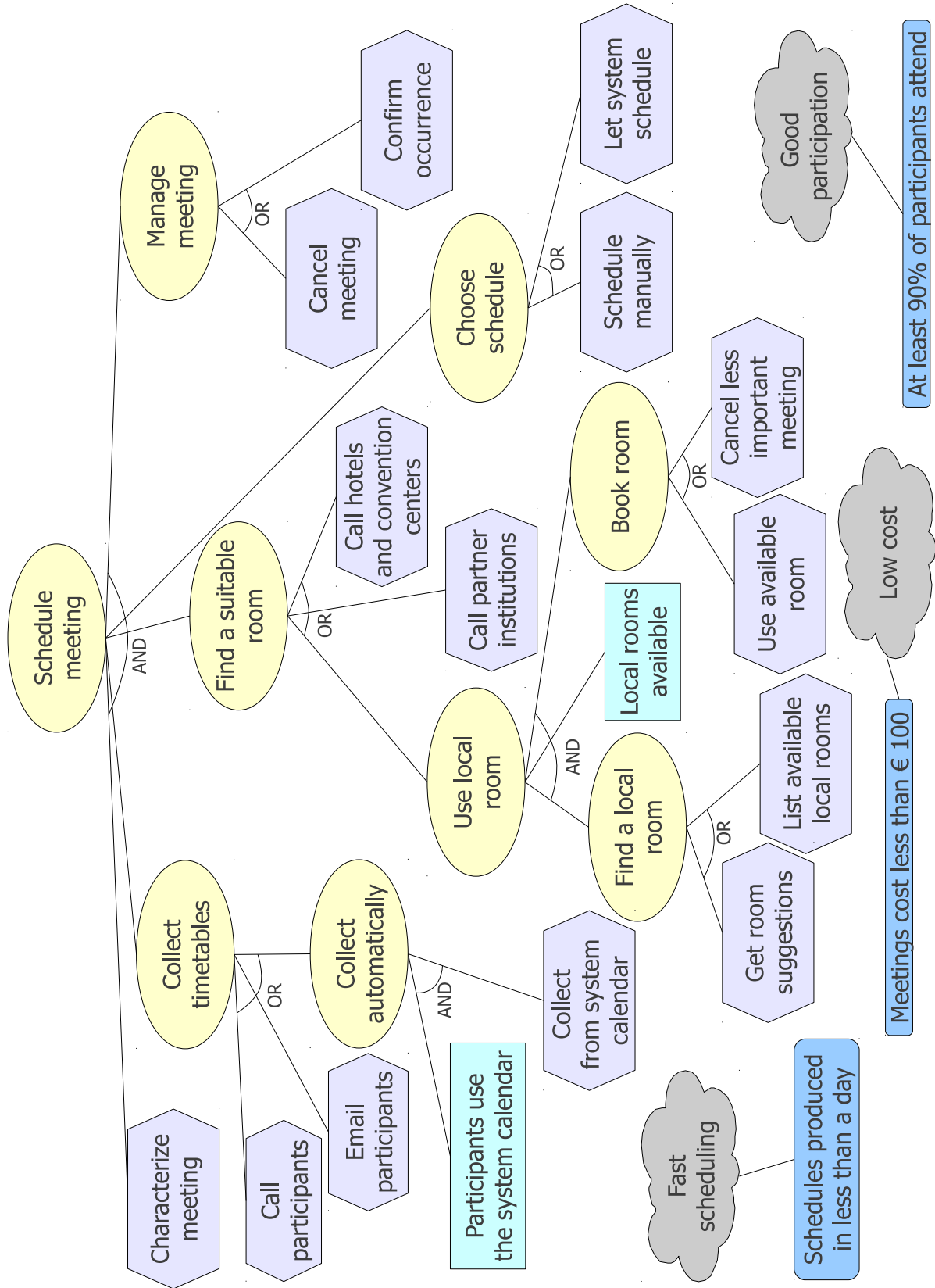
Figure 2.6: Final specification for the meeting scheduler, with added variability.
