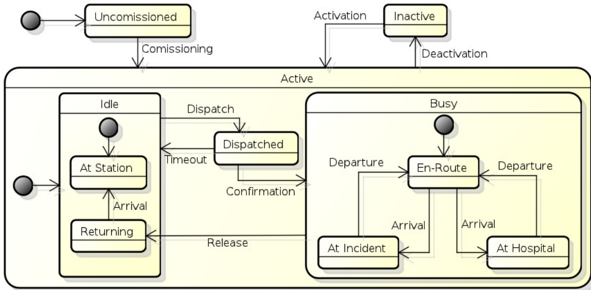
Figure 7.1: State-machine diagram for Ambulances.
