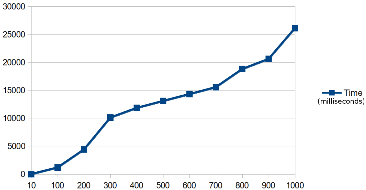
Figure 6.5: Results of the scalability tests of Zanshin .
