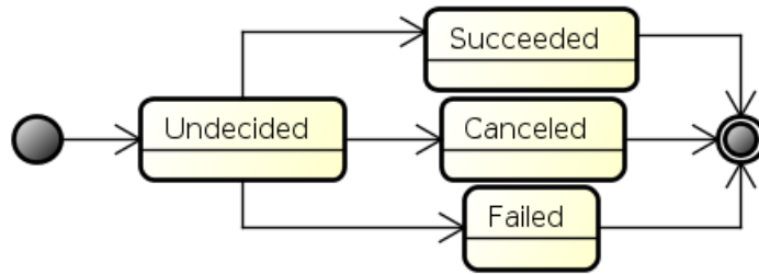
Figure 3.1: States assumed by GORE elements at runtime.
