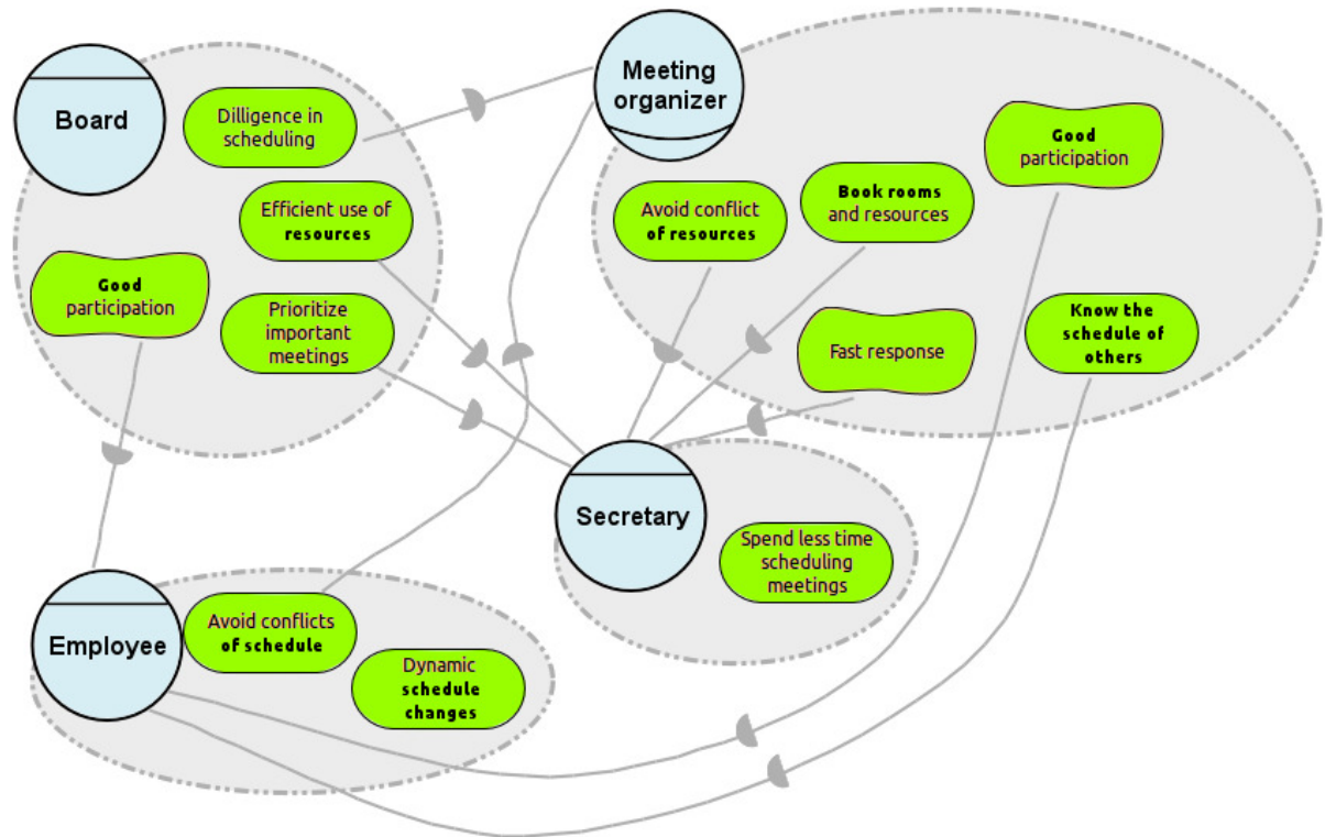
Figure 2.2: An i^* -like diagram depicting the strategic goals of the stakeholders.
