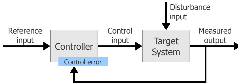
Figure 2.7: Simplified block diagram of a control system based on [Hellerstein et al., 2004].
