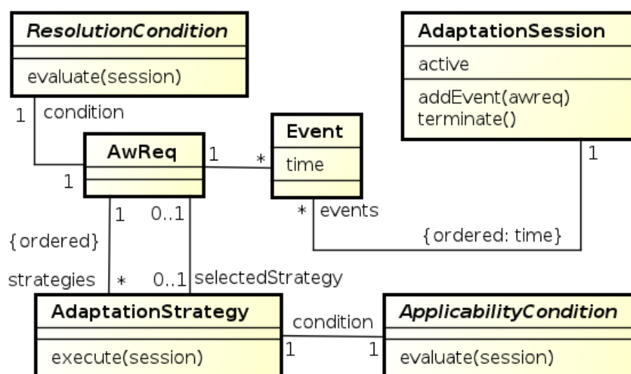
Figure 6.4: Entities involved in the ECA-based adaptation process.
