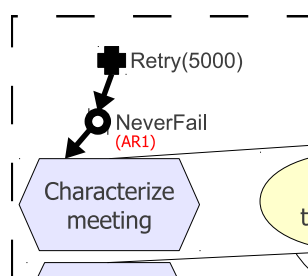
Figure 3.4: Graphical representation of an adaptation strategy in response to an AwReq failure.
