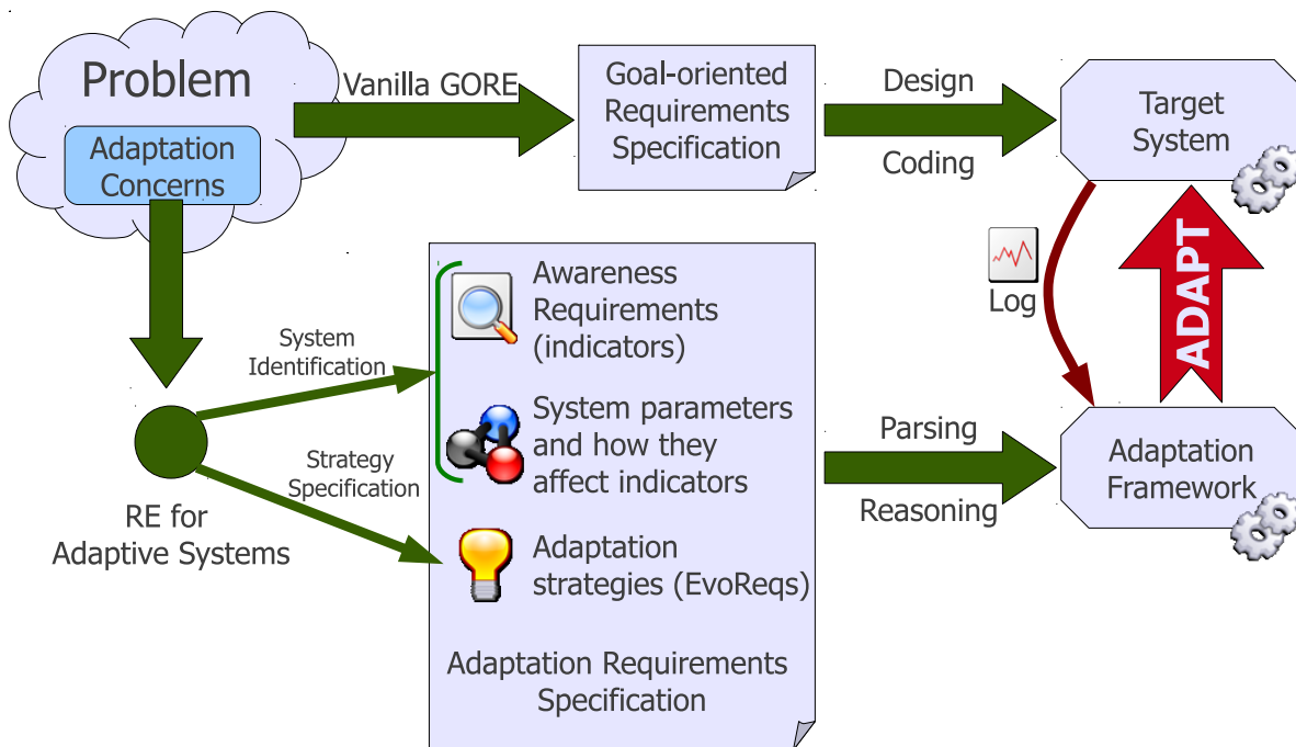
Figure 5.1: Overview of the Zanshin approach for the design of adaptive systems.
