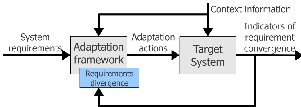
Figure 2.8: View of an adaptive system as a feedback control system.
