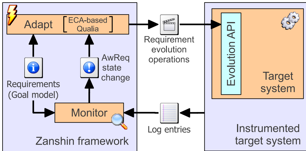
Figure 6.1: Overview of the Zanshin framework.
