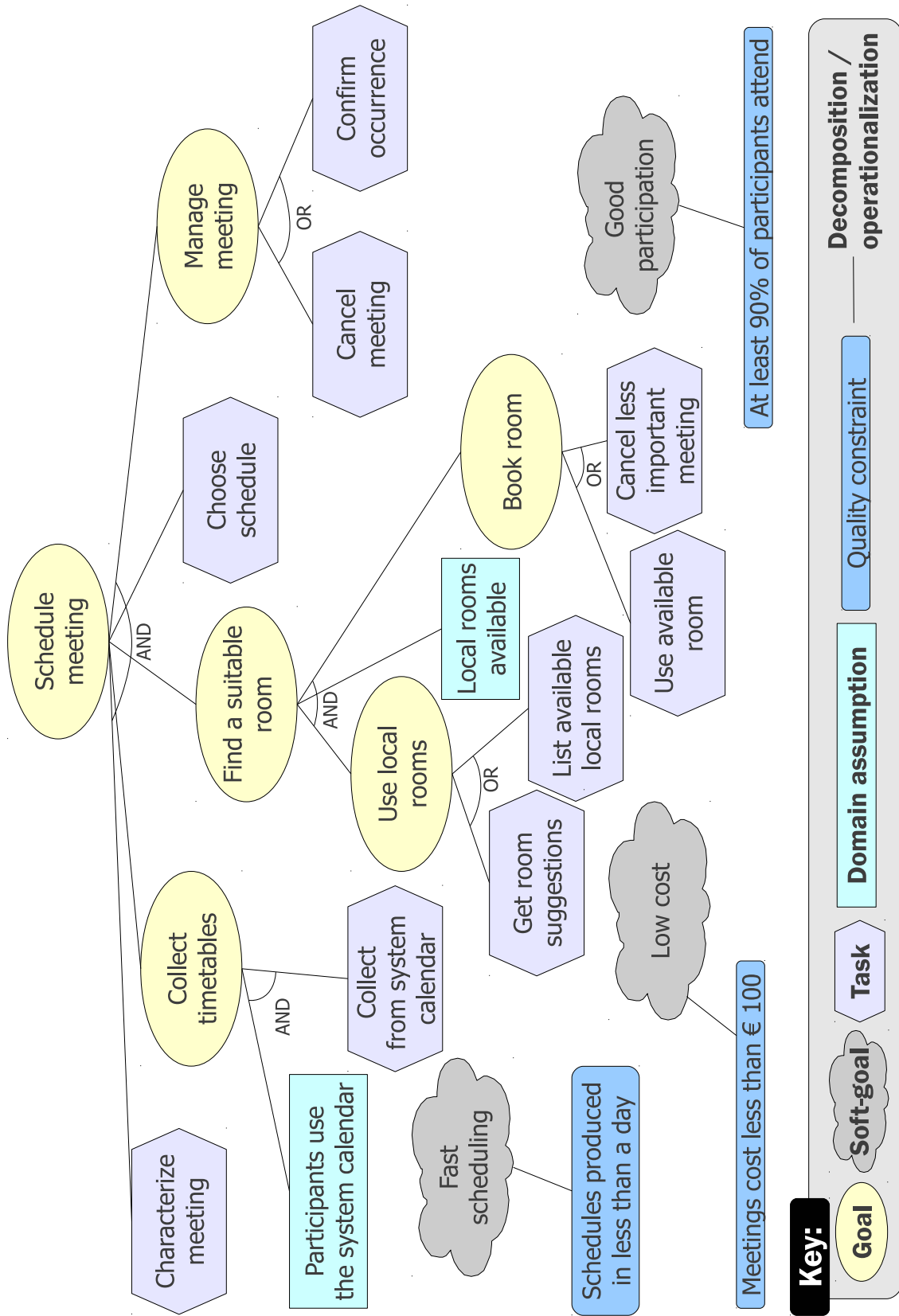
Figure 2.5: Initial specification for the meeting scheduler.
