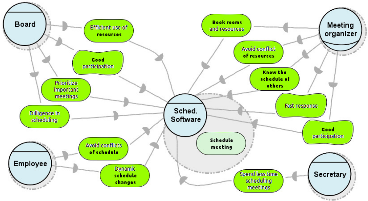
Figure 2.4: Strategic Dependencies for the meeting scheduler system-to-be.
