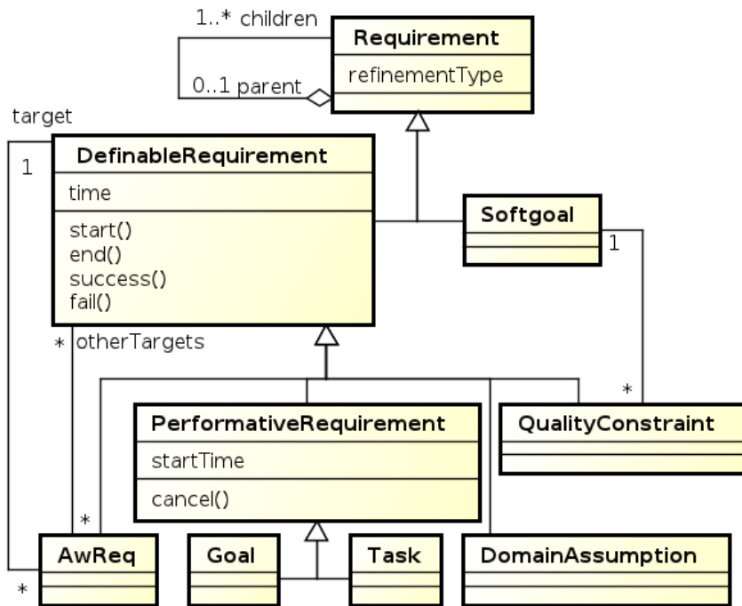
Figure 3.2: Class model for requirements in GORE-based specifications.
