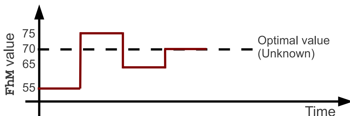
Figure 4.5: A scenario of use of the Oscillation Algorithm in the Meeting Scheduler.
