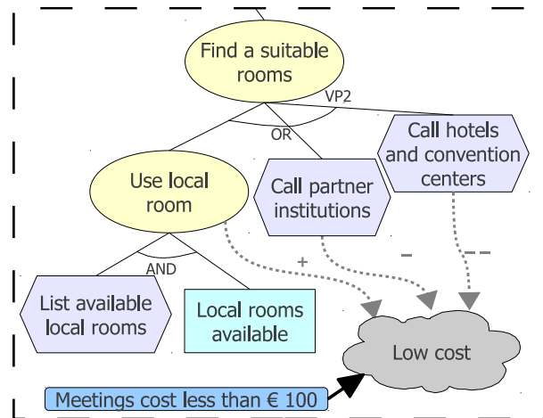
Figure 5.2: Contribution links may help identifying differential relations in variation points.
