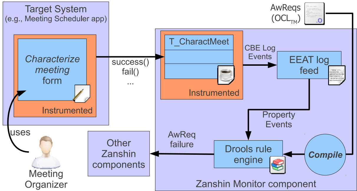
Figure 6.2: Overview of Zanshin 's Monitor component.
