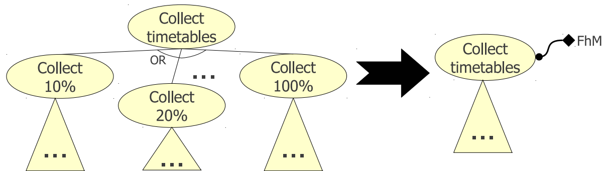
Figure 4.2: Using a control variable as an abstraction over families of subgraphs.
